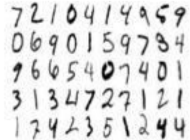
Image Recognition
